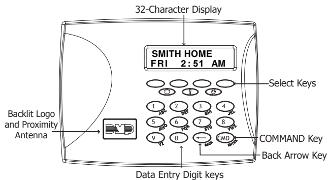
DMP 9000 Series Wireless Keypad
